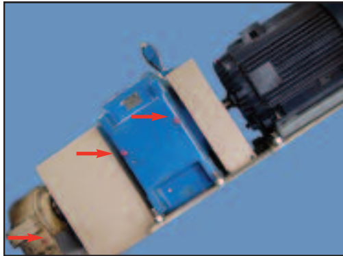
Pictured above is a condition monitoring system showing red caps on sensor mounts for the Motor, Gearbox, and Bearing on this drive system.
